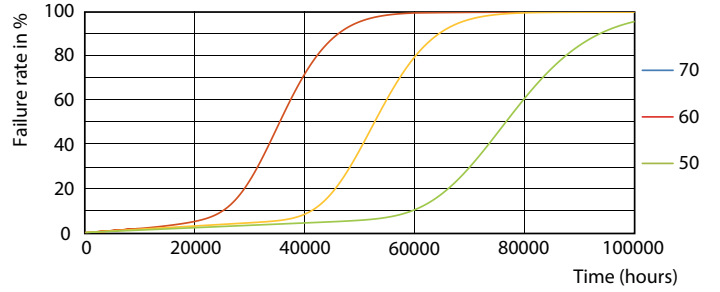
Lumen Maintenance Diagram - MAS LEDtube 600mm HO 8W830 T8 FailureRate
