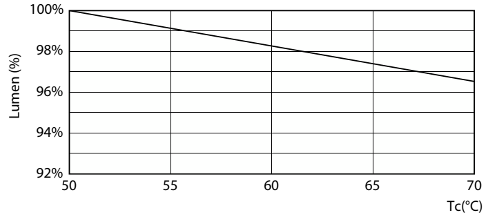
Life Expectancy Diagram Lumen Maintenance Diagram - MAS LEDtube 600mm HO 8W830 T8
